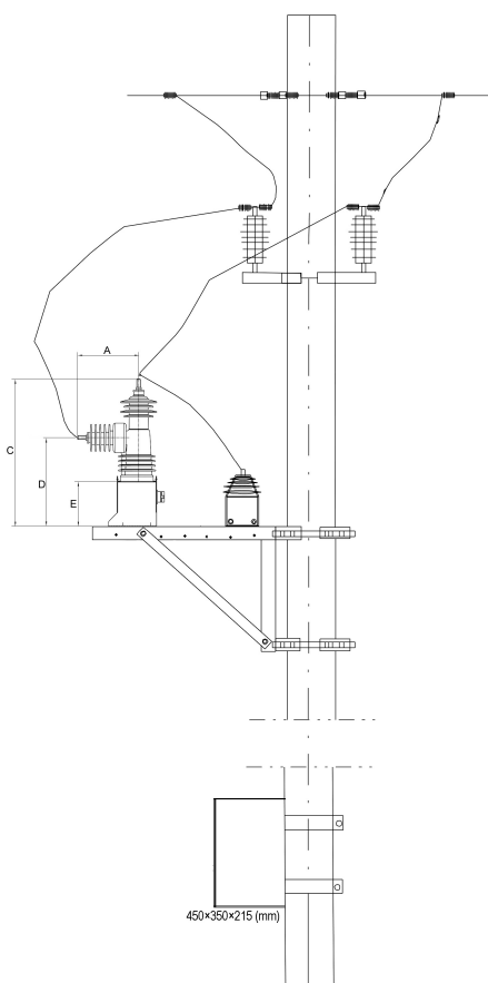
Pole mount
