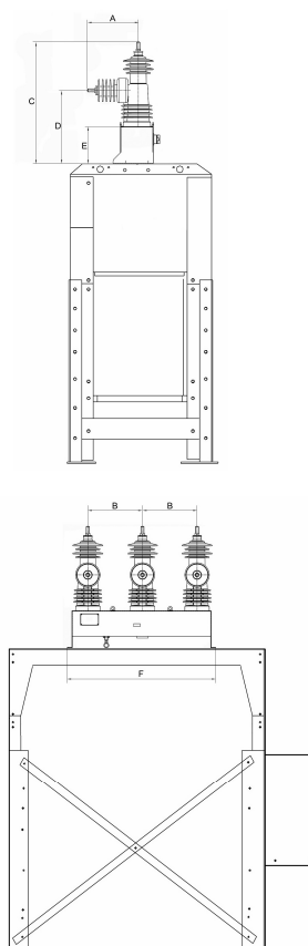
Substation mount
