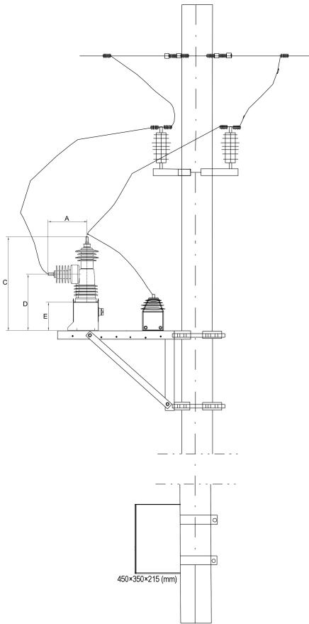
Pole mount
