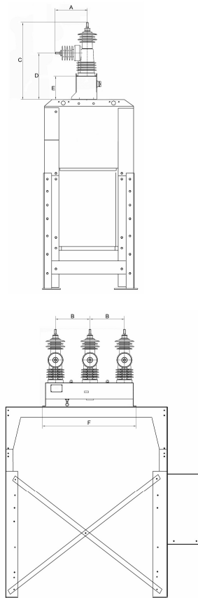
Substation mount
